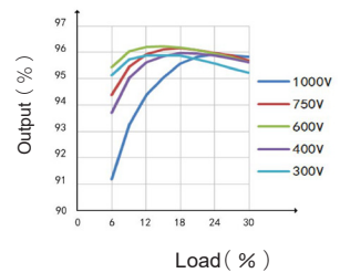
Output efficiency curve
